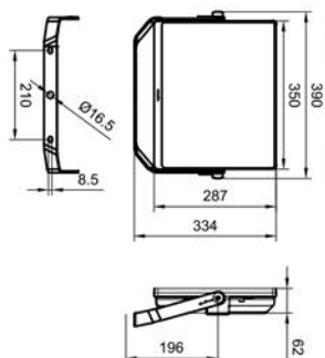
BVP173/174/175/176 Smartbright
