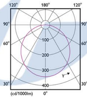
Light Distribution Diagram - DN020B G3 LED20/WW 23W 220-240V D200 GM
