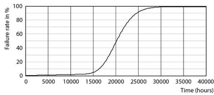
Life Expectancy Diagram - DN020B G3 LED20/WW 23W 220-240V D200 GM
