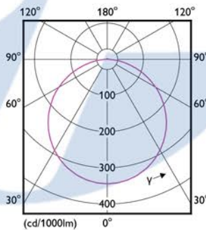
Light Distribution Diagram - DN020B G3 LED12/WW 14W 220-240V D150 MY
