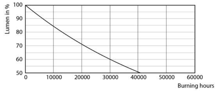
Lumen Maintenance Diagram - DN020B G3 LED12/WW 14W 220-240V D150 MY
