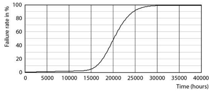
Life Expectancy Diagram - DN020B G3 LED12/WW 14W 220-240V D150 MY
