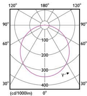
Light Distribution Diagram - DN020B G3 LED12/NW 14W 220-240V D150 MY
