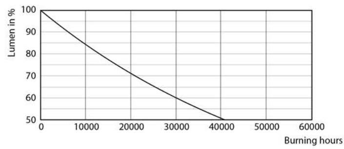
Lumen Maintenance Diagram - DN020B G3 LED12/NW 14W 220-240V D150 MY
